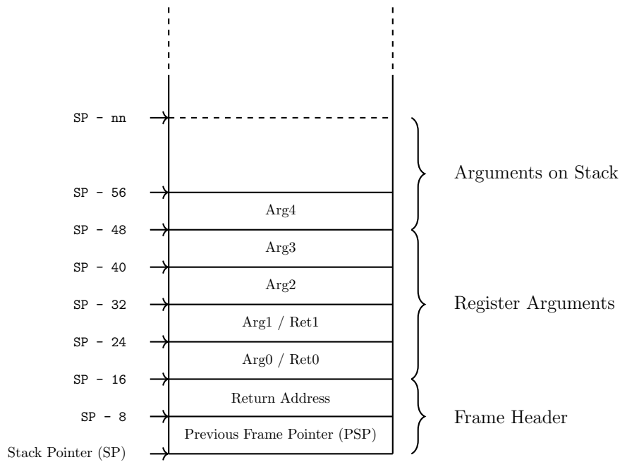
Figure 19: Argument Passing
