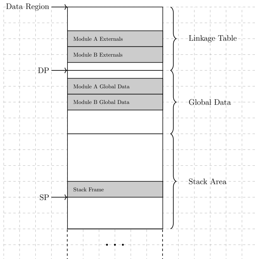
Figure 20: Linkage Table
