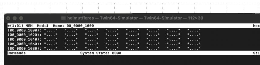
Figure 33: Simulator MEM Window - Ascii
