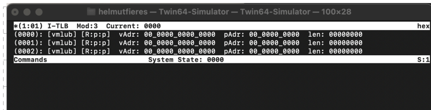
Figure 29: Simulator CPU Window - TLB
