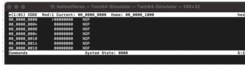
Figure 35: Simulator MEM Window - Code
