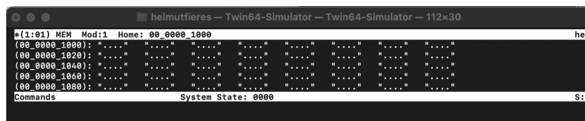
Figure 47: Simulator Memory Window ASCII
