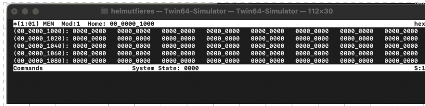
Figure 31: Simulator MEM Window - Hex32
