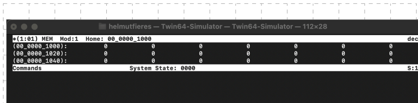
Figure 33: Simulator MEM Window - Decimal
