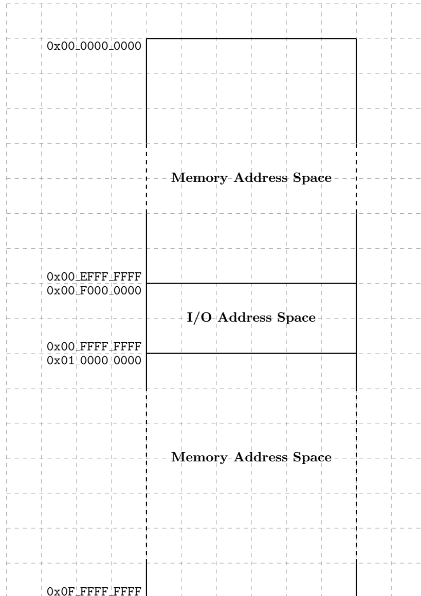
Figure 8: Physical Memory Address Range
