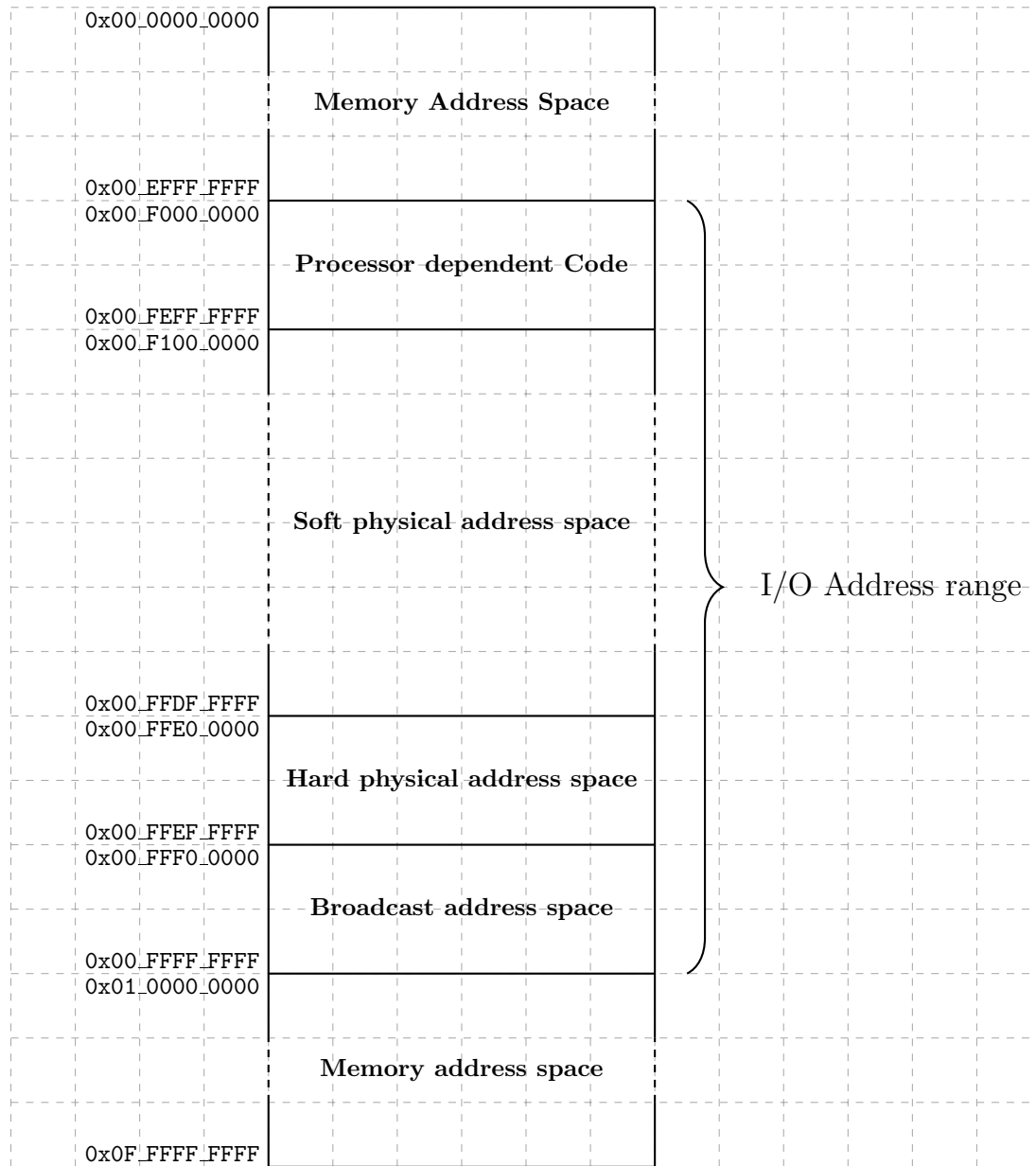
Figure 9: I/O Memory Address Range
