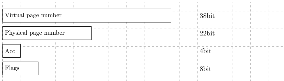
Figure 6: Tlb info
