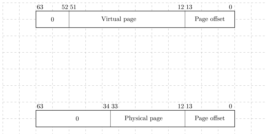
Figure 10: Address translation
