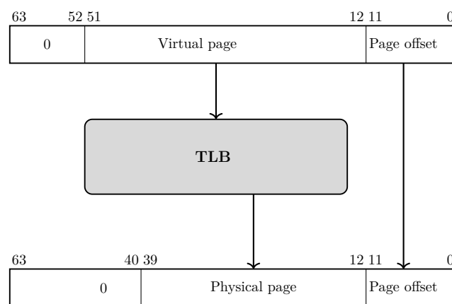
Figure 10: Address translation
