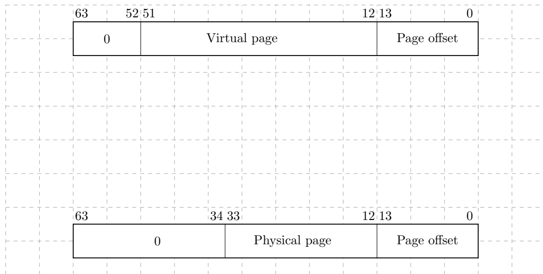
Figure 9: Address translation
