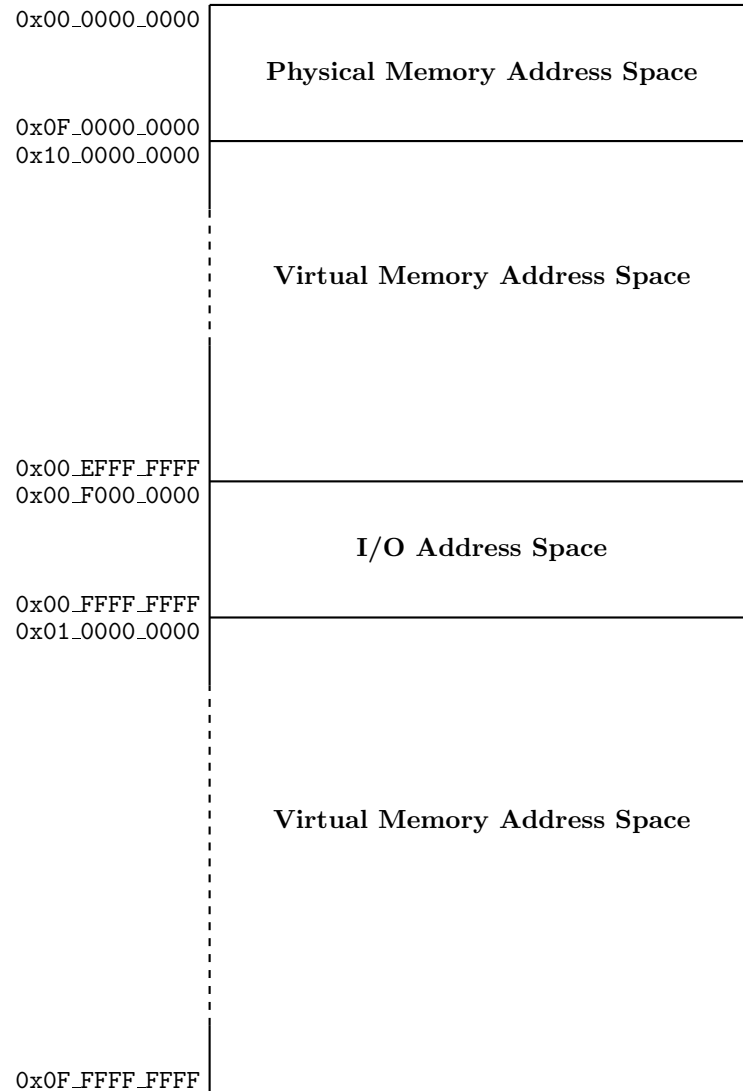
Figure 9: Physical Memory Address Range
