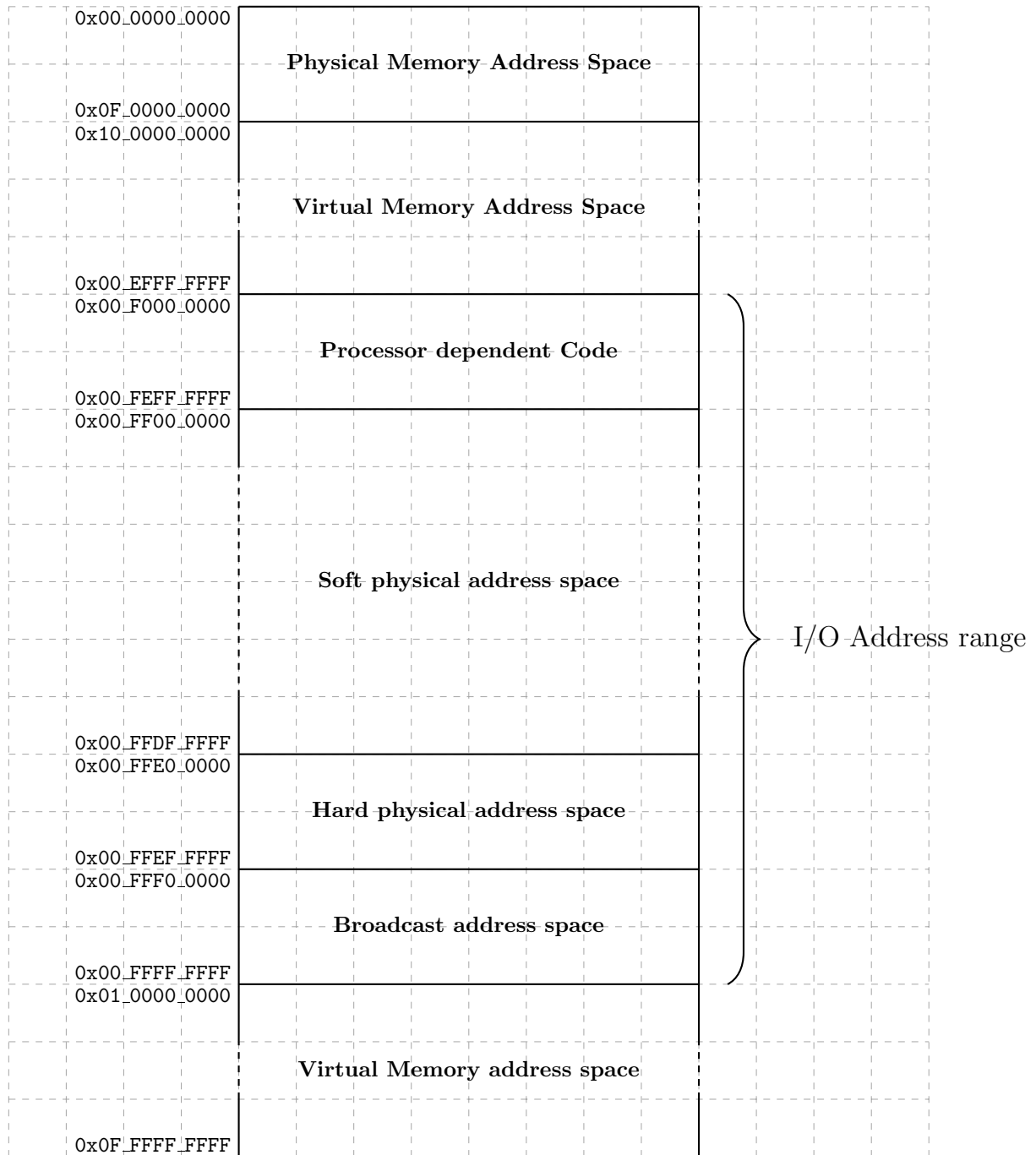
Figure 13: I/O Memory Address Range
