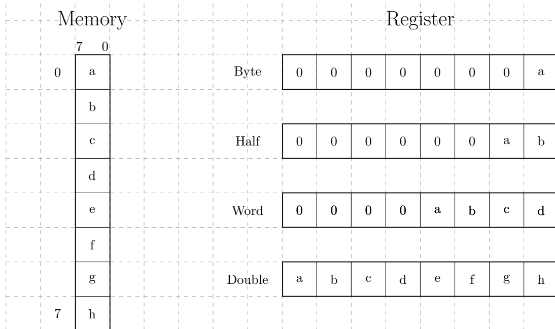
Figure 6: Big endian mode
