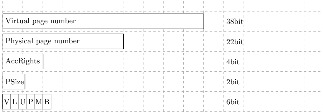
Figure 7: Tlb info
