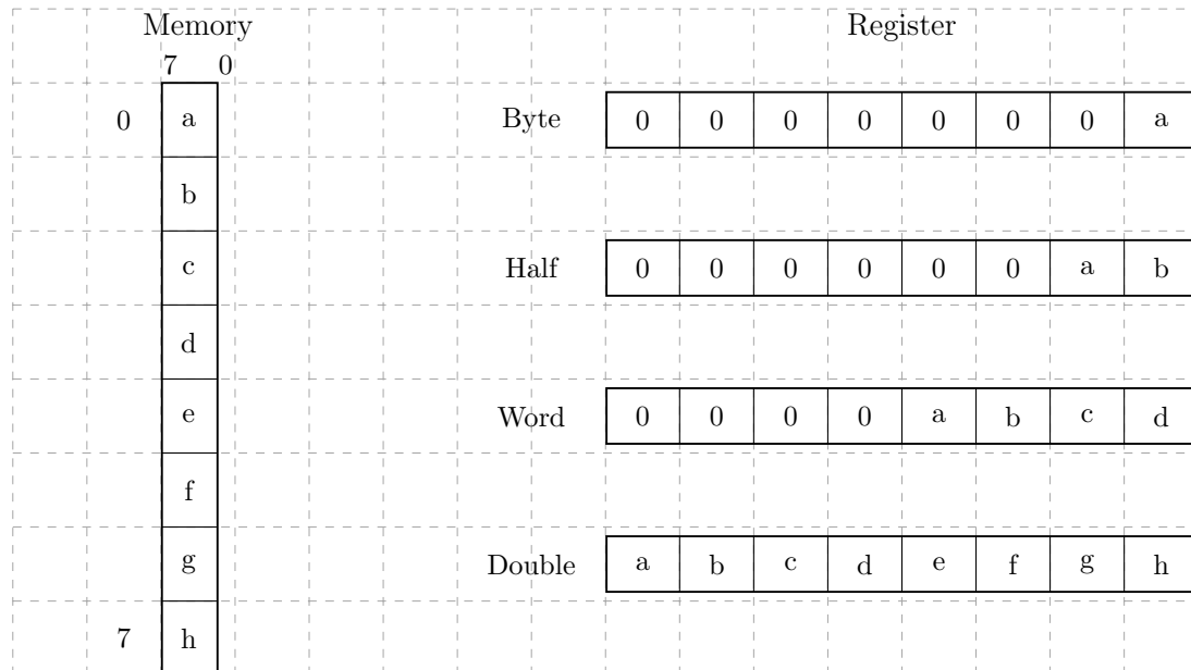
Figure 6: Big endian mode
