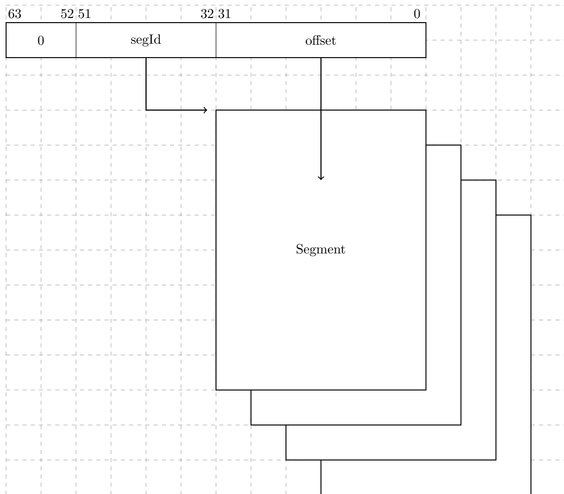
Figure 8: Virtual Memory Address Range
