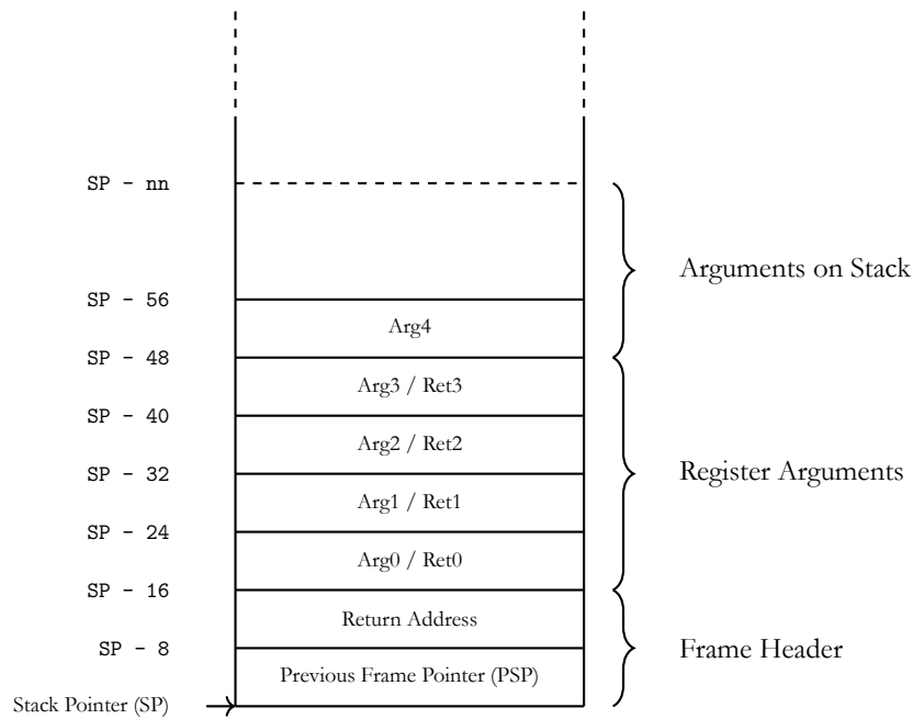
Figure 23: Argument Passing
