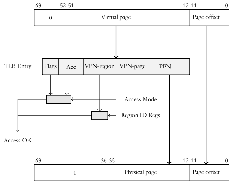
Figure 13: Address translation
