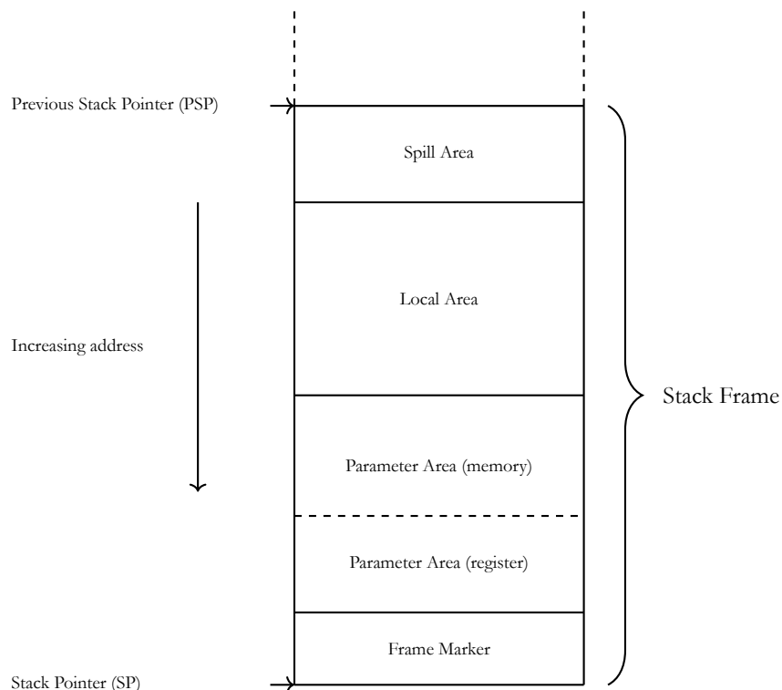
Figure 21: Stack Frame
