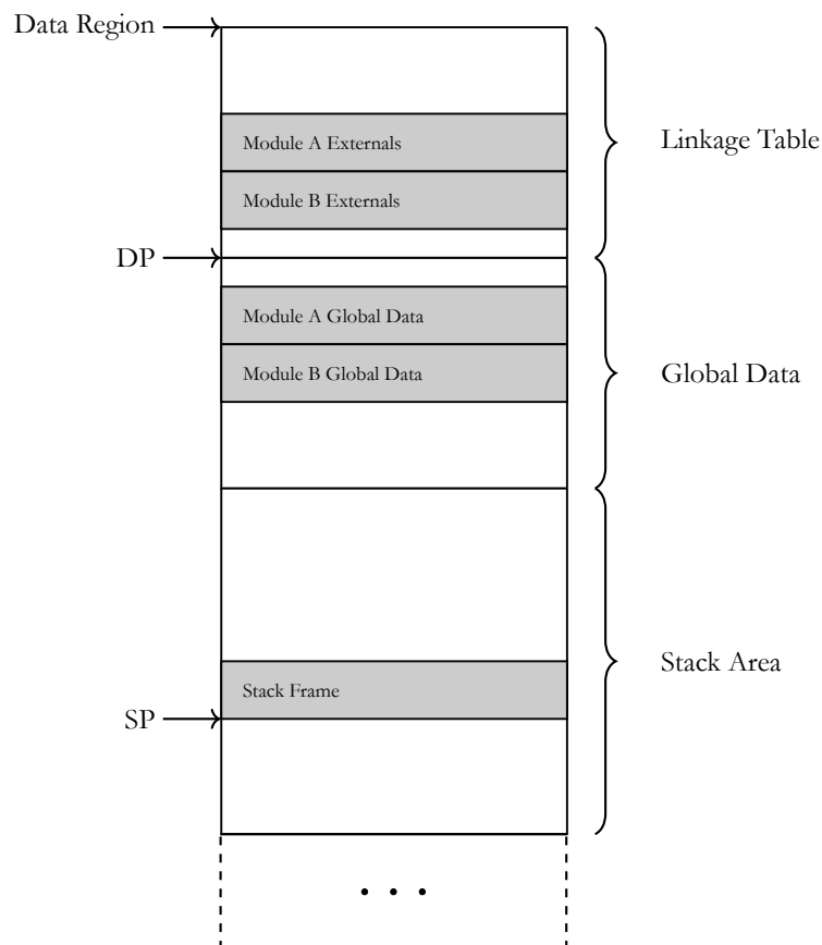
Figure 24: Linkage Table
