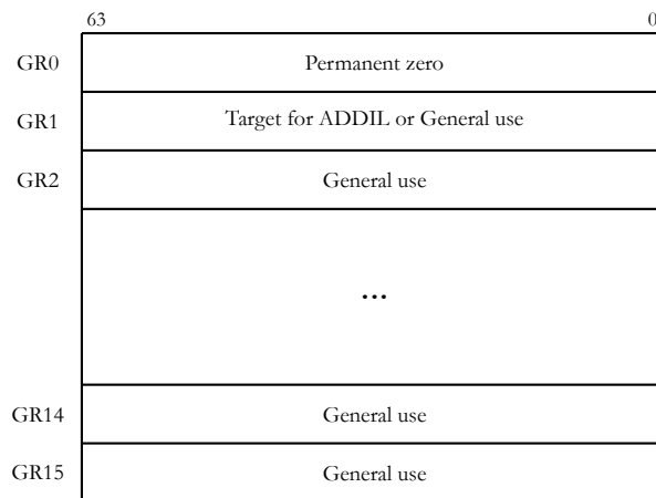
Figure 1: General registers
