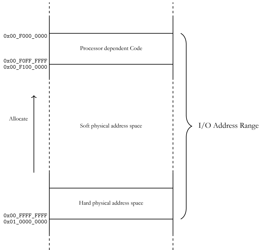
Figure 14: I/O Address Space
