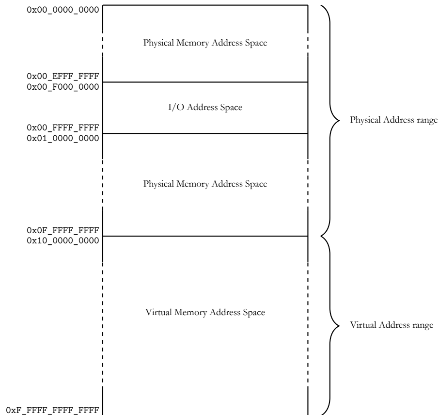
Figure 9: Memory Address Ranges
