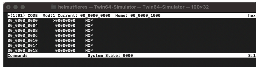
Figure 34: Simulator Memory Window - Code
