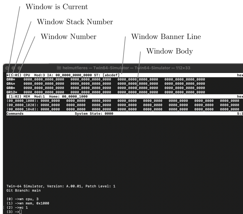
Figure 23: Simulator Environment Screen
