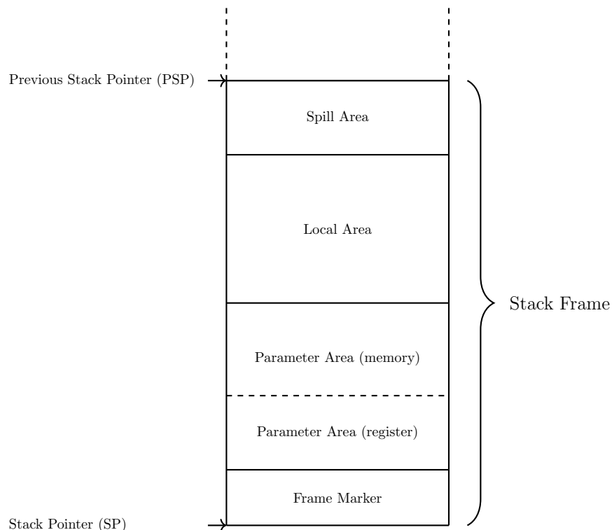
Figure 16: Stack Frame
