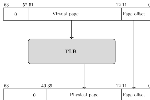
Figure 10: Address translation
