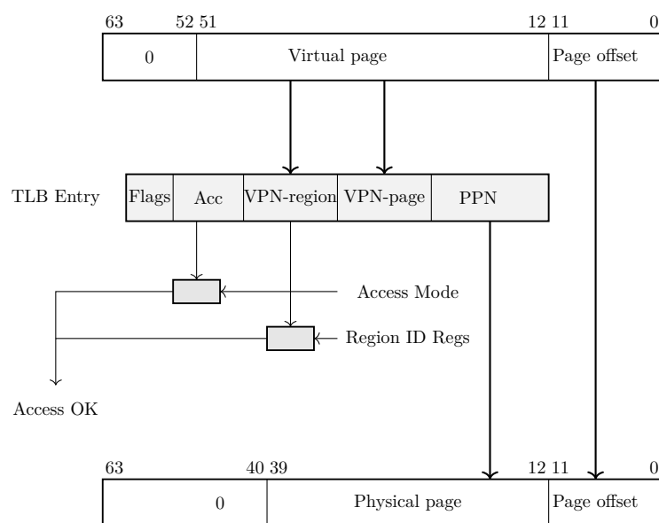
Figure 13: Address translation
