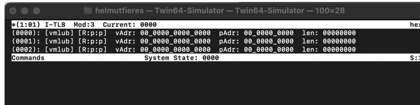
Figure 31: Simulator TLB Window
