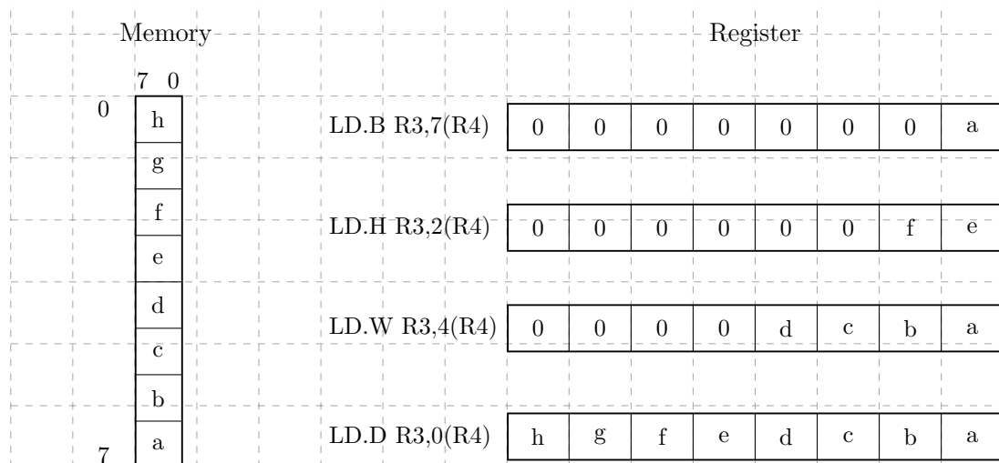
Figure 7: Big endian mode
