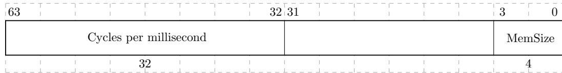
Figure 4: Processor Configuration Register
