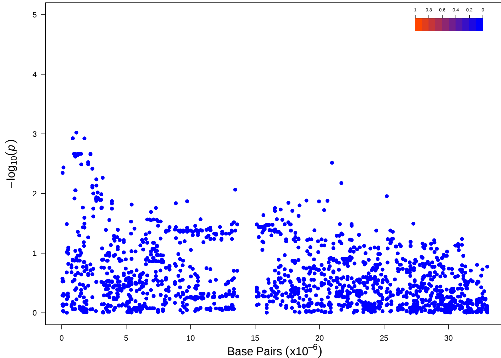
Chromosome 12
