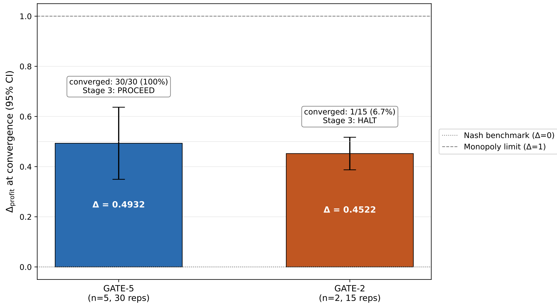
\Delta_{\text{profit}} comparable across n=5 and n=2 ; convergence rate diverges sharply
