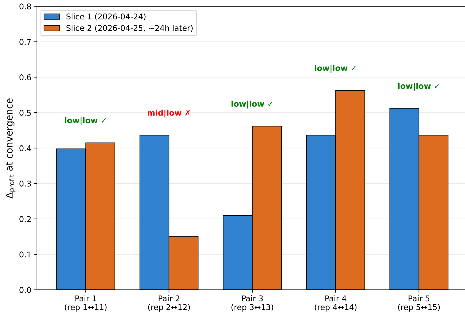
Within-Host-A pairwise: 4/5 regime match across ~24h gap
