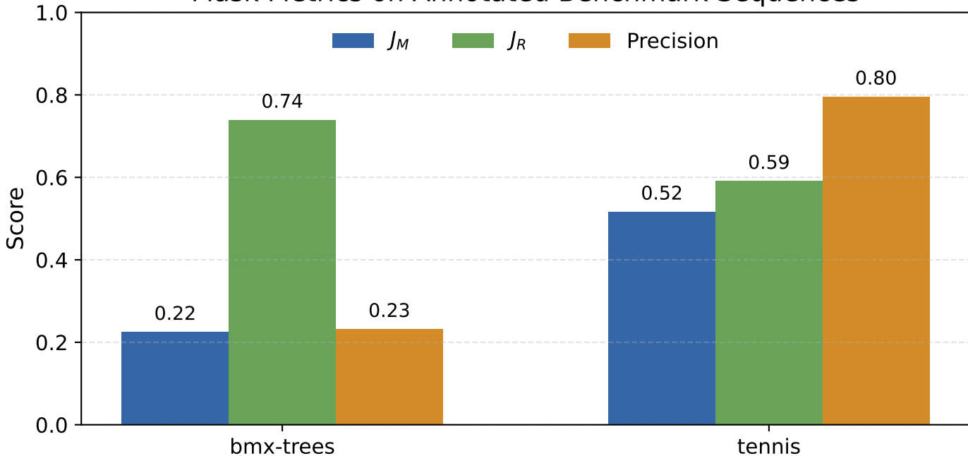
Mask Metrics on Annotated Benchmark Sequences
