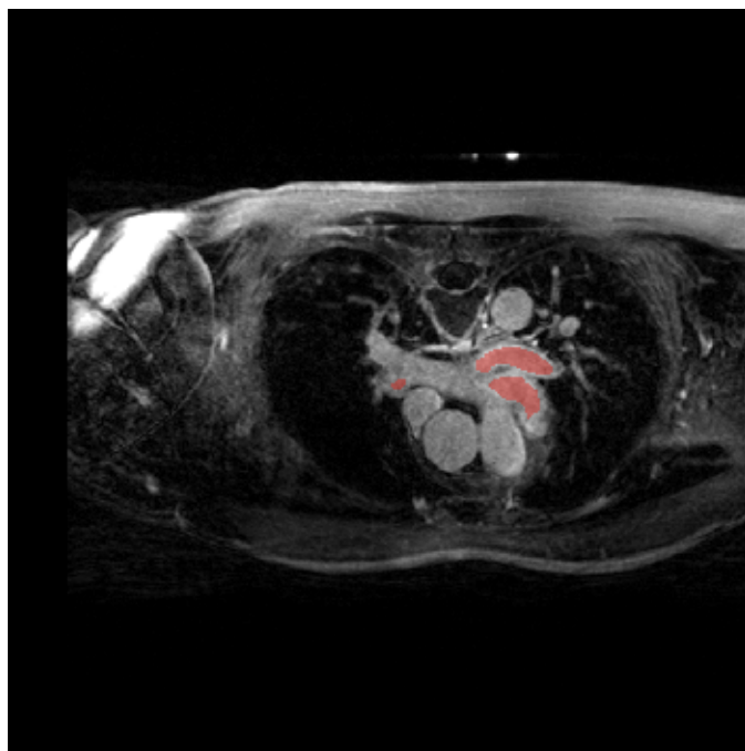
3D U-Net
