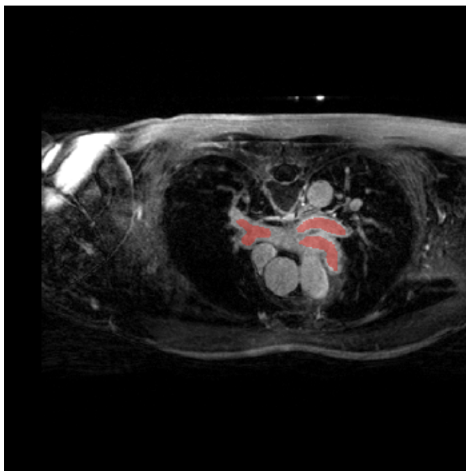
2D U-Net
