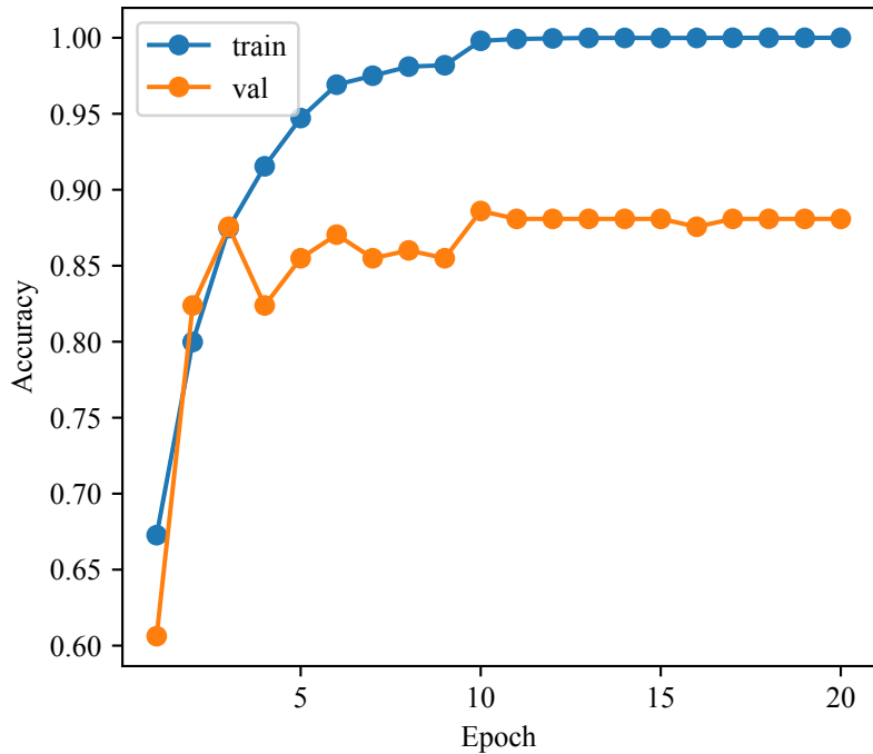
Accuracy
