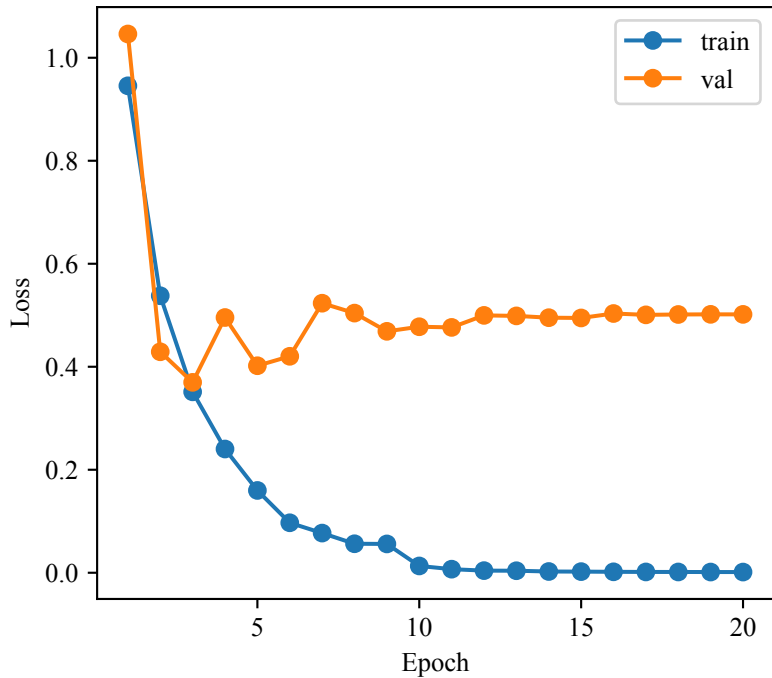
Cross-entropy loss
