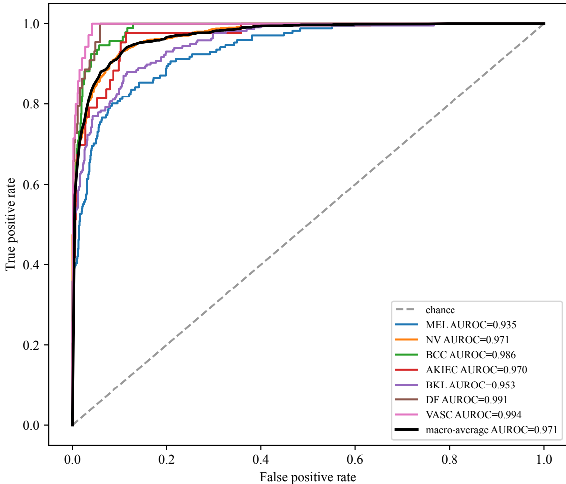
Test one-vs-rest ROC
