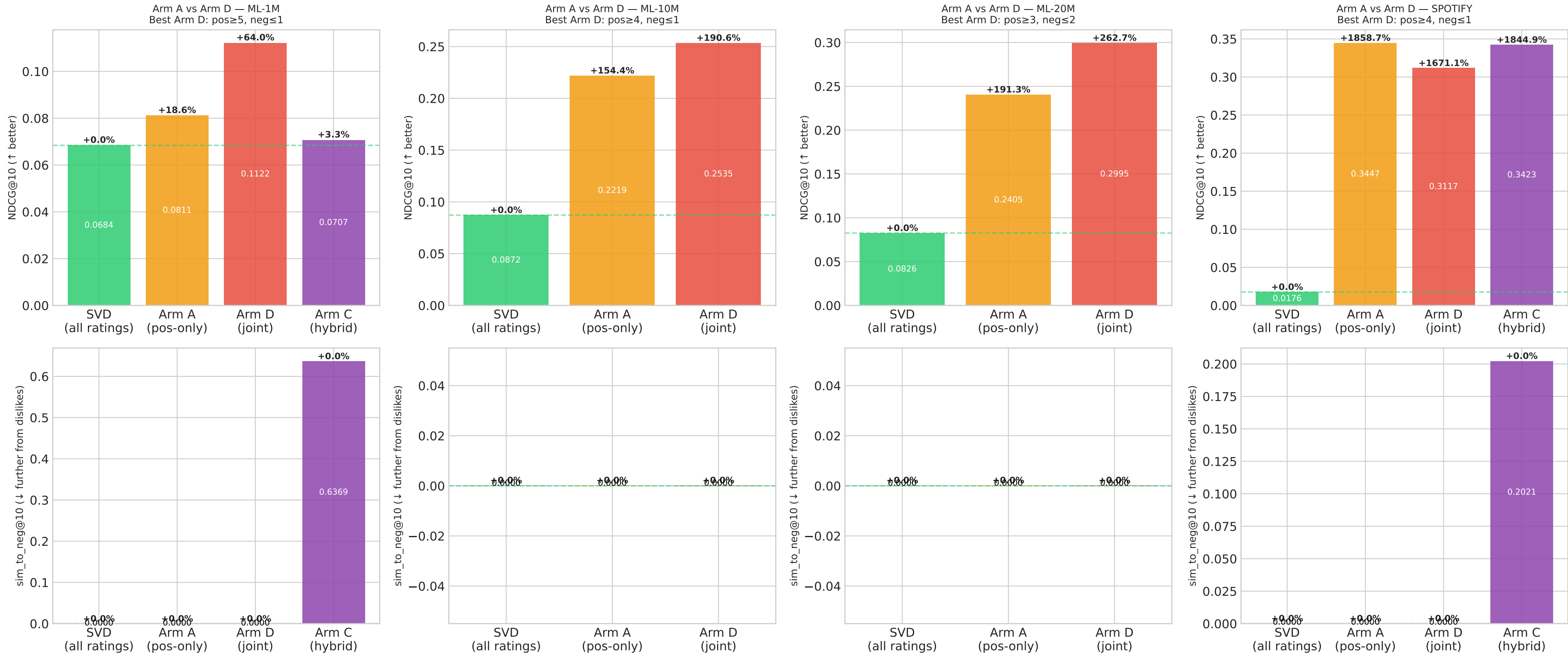
Fig — Arm A vs Arm D: Does joint positive-negative training improve ranking? Arm D trains SVD on binary targets (pos=1.0, neg=0.0). \Delta\% vs full-rating SVD baseline.
