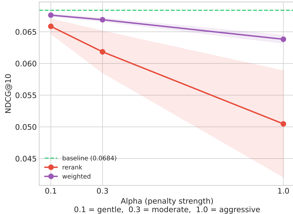
Fig 4 — Effect of Alpha on NDCG (ML-1M) Is there a penalty level that helps without hurting?
