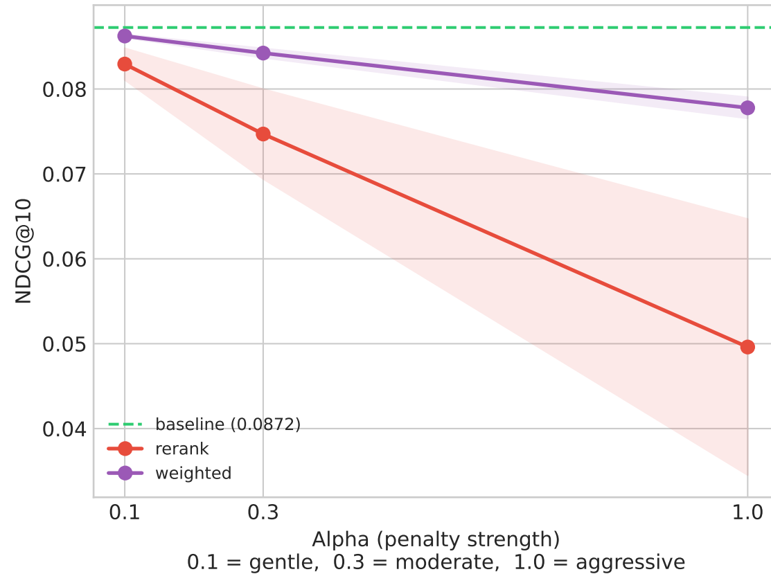
Fig 4 — Effect of Alpha on NDCG (ML-10M) Is there a penalty level that helps without hurting?
