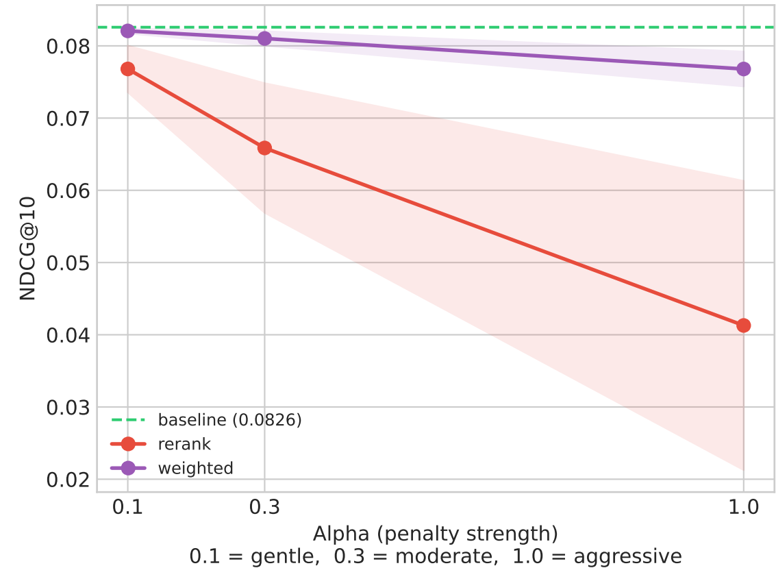
Fig 4 — Effect of Alpha on NDCG (ML-20M) Is there a penalty level that helps without hurting?
