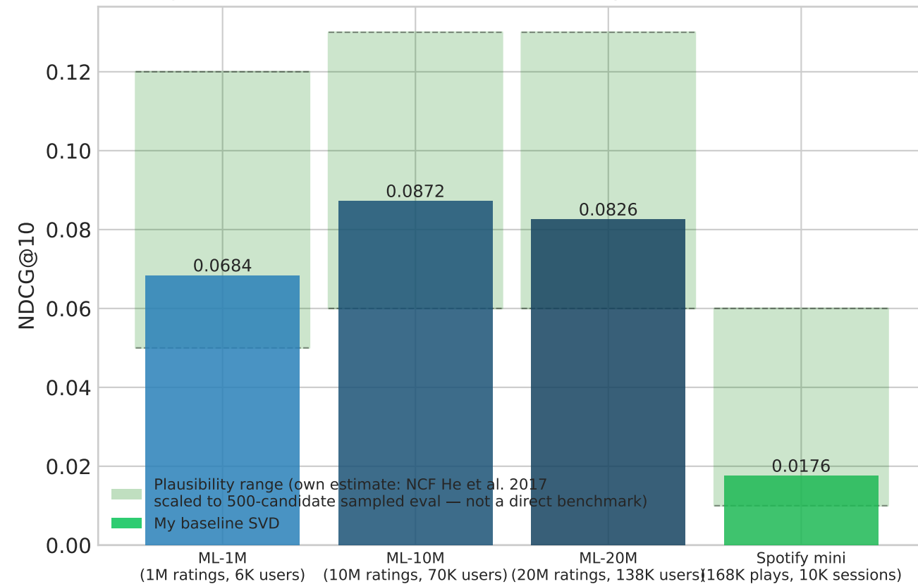
Fig 1b — My NDCG@10 vs Plausibility Range (green band = heuristic estimate, not a published benchmark)
