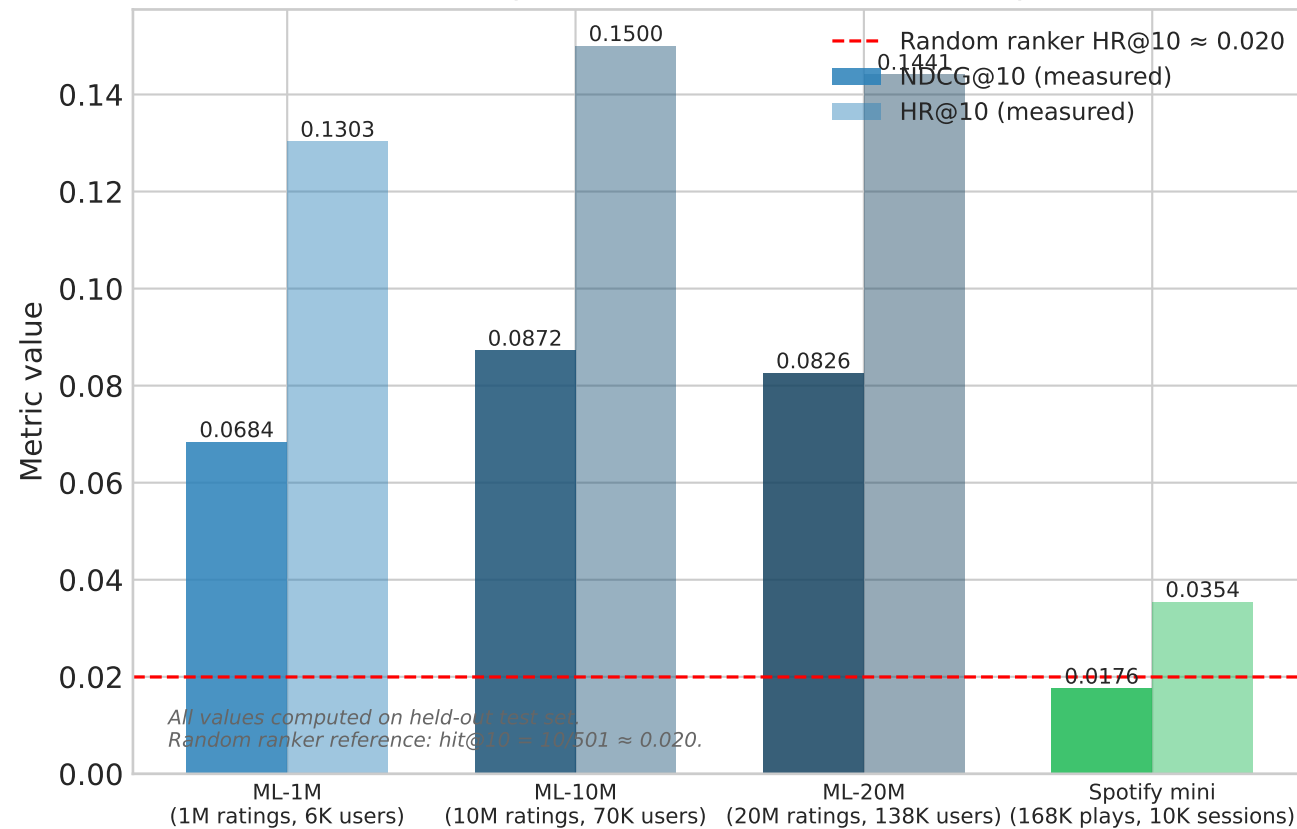
Fig 1a — Baseline SVD: NDCG@10 and HR@10 (501 sampled candidates, random LOO split)
