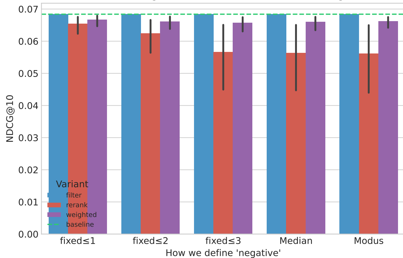
Fig 5a — NDCG@10 by Threshold (ML-1M) Broader negative definition → more NDCG damage
