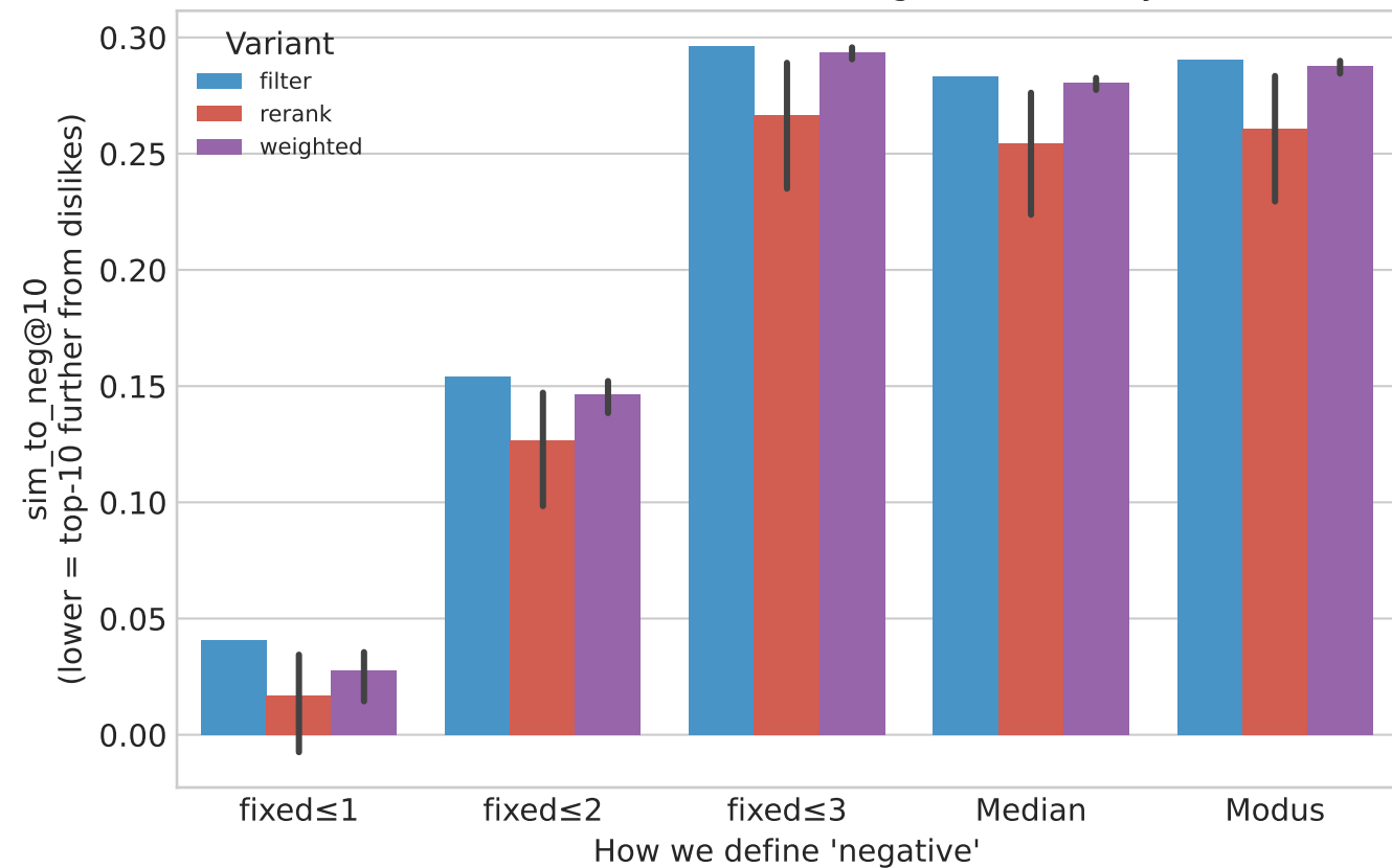
Fig 5b — sim_to_neg@10 by Threshold (ML-1M) Broader definition also reduces negative similarity more
