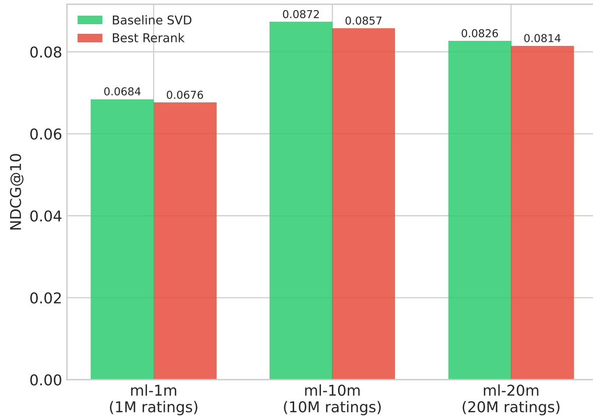
Fig 6a — Baseline vs Best Rerank across Sizes Does more data help, and does rerank help more?
