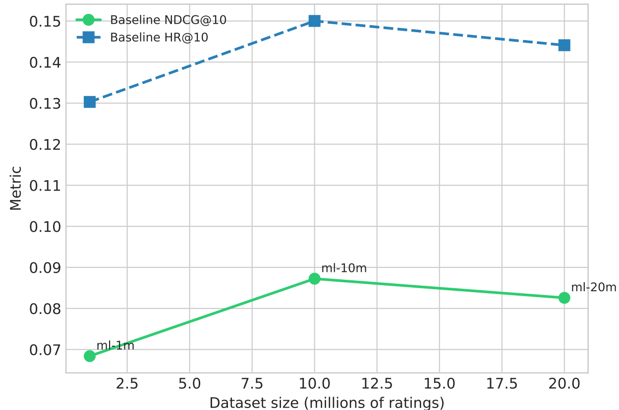
Fig 6b — Does SVD Improve with More Data? (each point = one MovieLens version)
