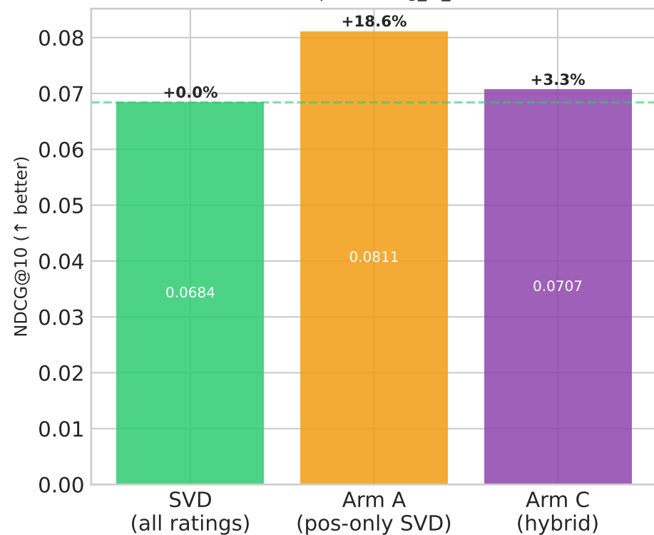
Arm A vs Arm C — ML-1M Best Arm C: pos \geq 3, neg_le_1, \alpha=0.05
