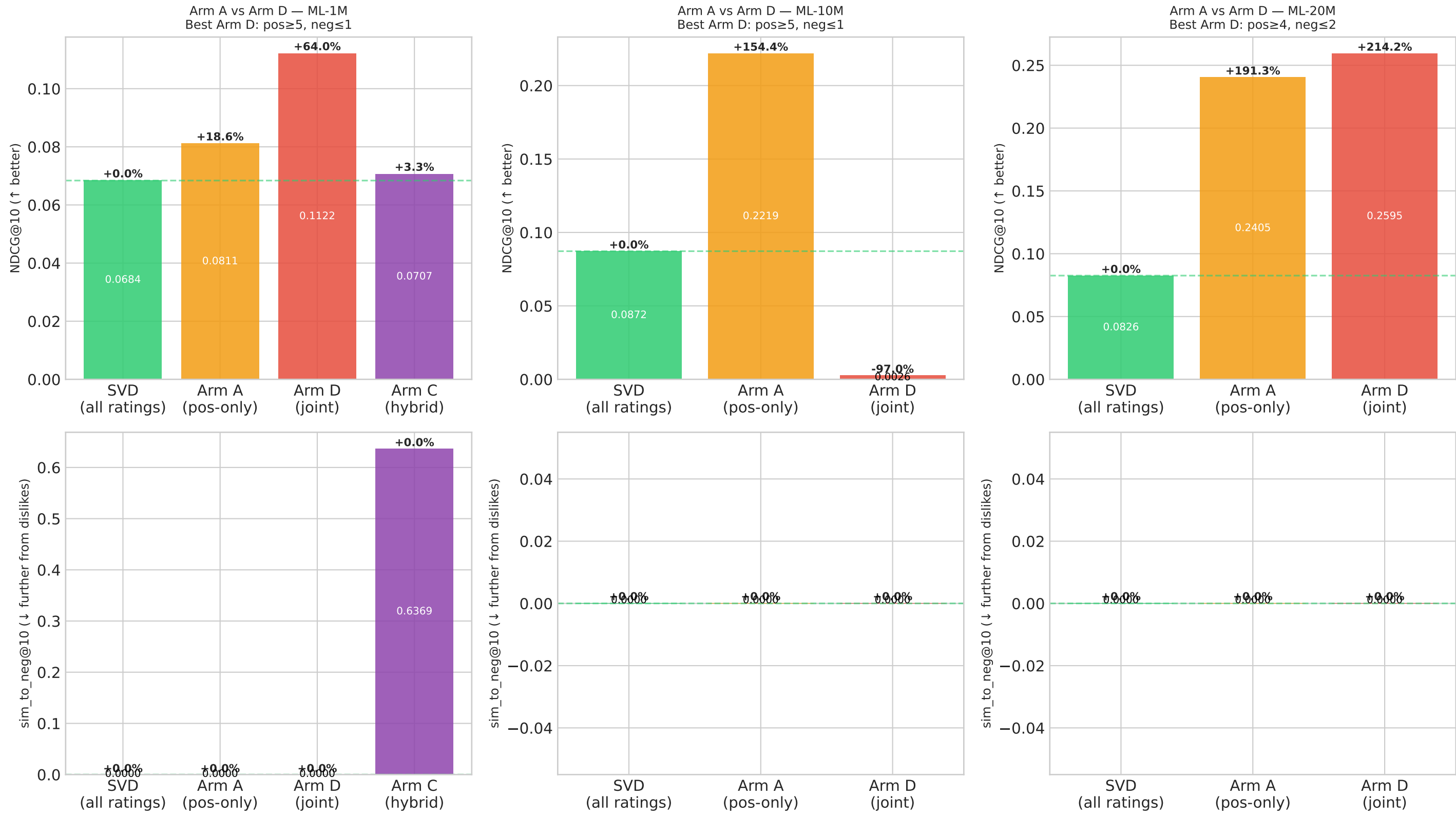
Fig — Arm A vs Arm D: Does joint positive-negative training improve ranking? Arm D trains SVD on binary targets (pos=1.0, neg=0.0). \Delta\% vs full-rating SVD baseline.
