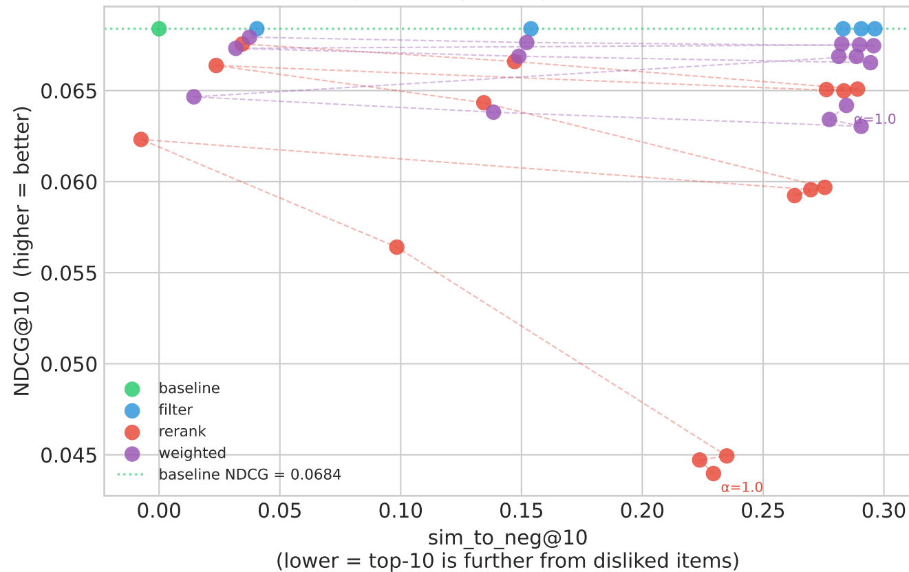
Fig 2 — The Core Tradeoff (ML-1M) Reducing similarity to negatives hurts NDCG
