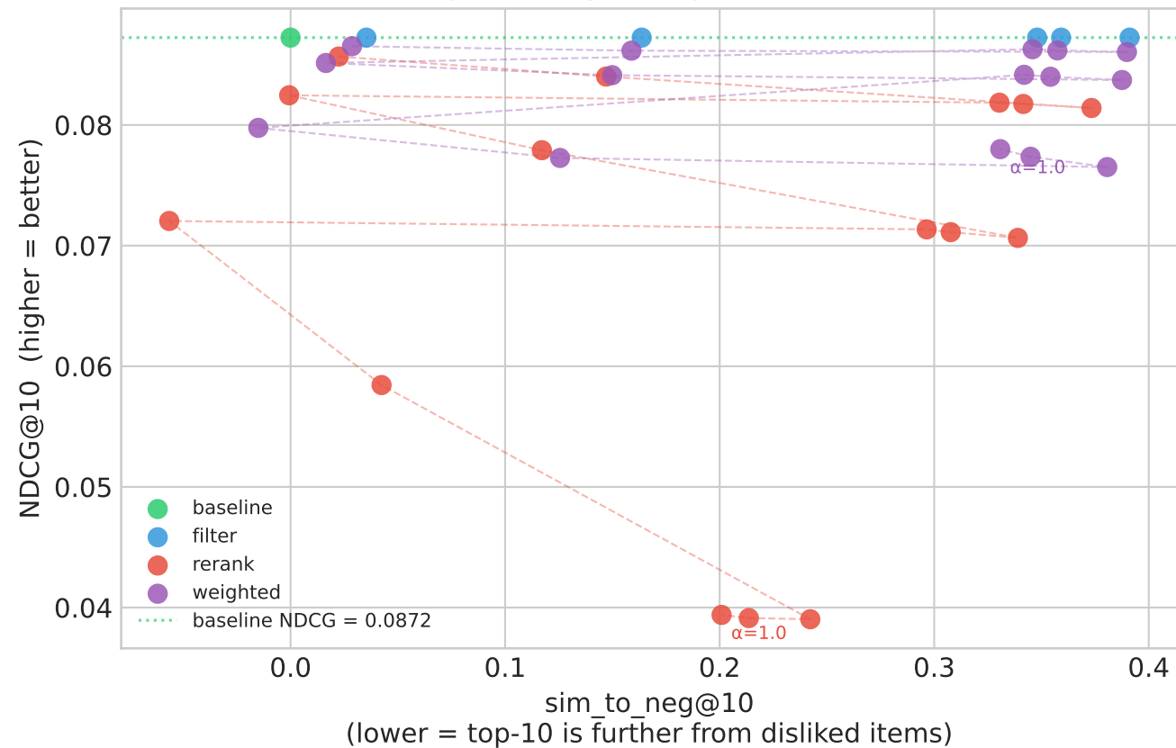
Fig 2 — The Core Tradeoff (ML-10M) Reducing similarity to negatives hurts NDCG
