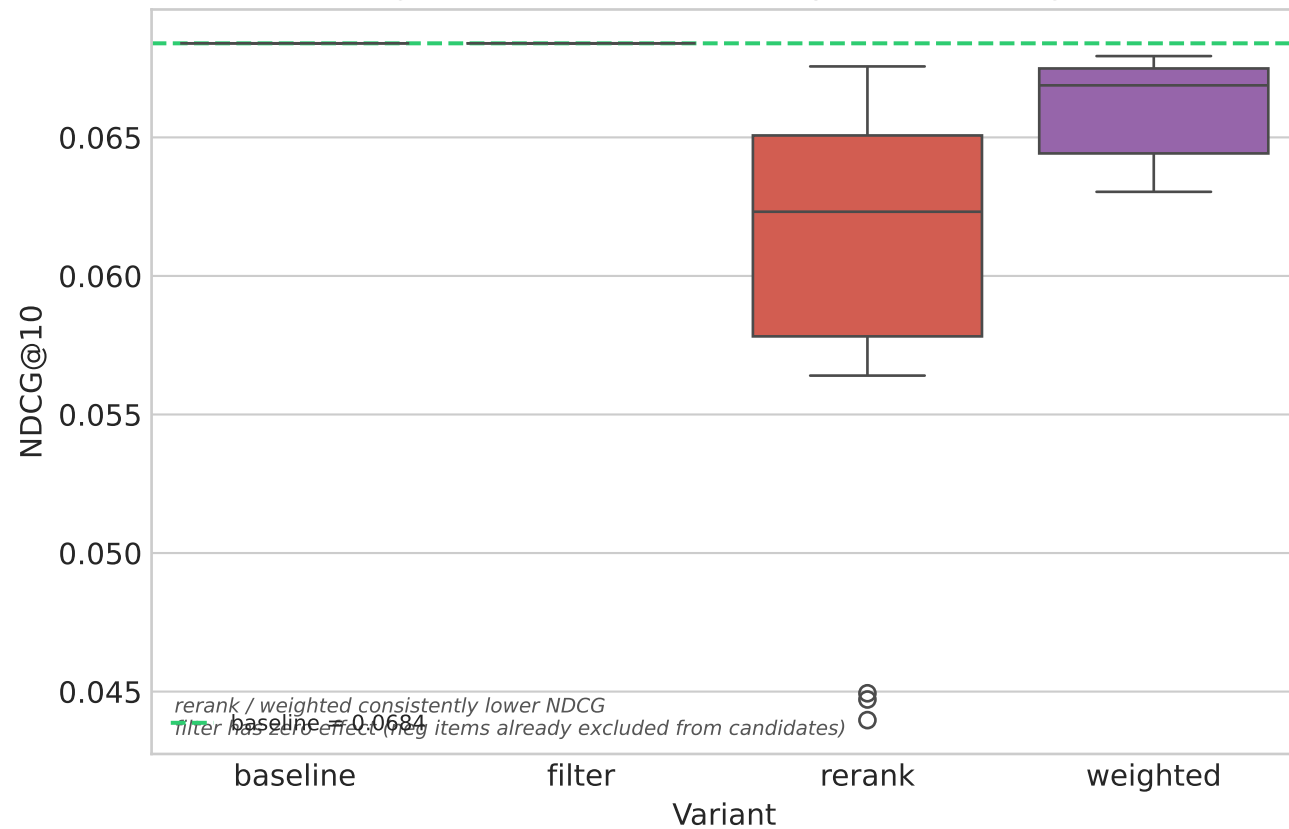
Fig 7 — MovieLens 1M — explicit star ratings
