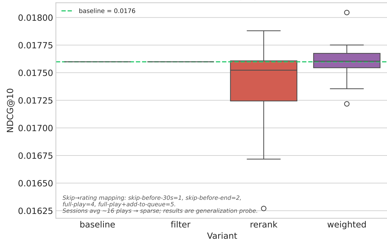
Fig 7 — Spotify MSSD — implicit skip signals (session = user, ~16 plays/session)
