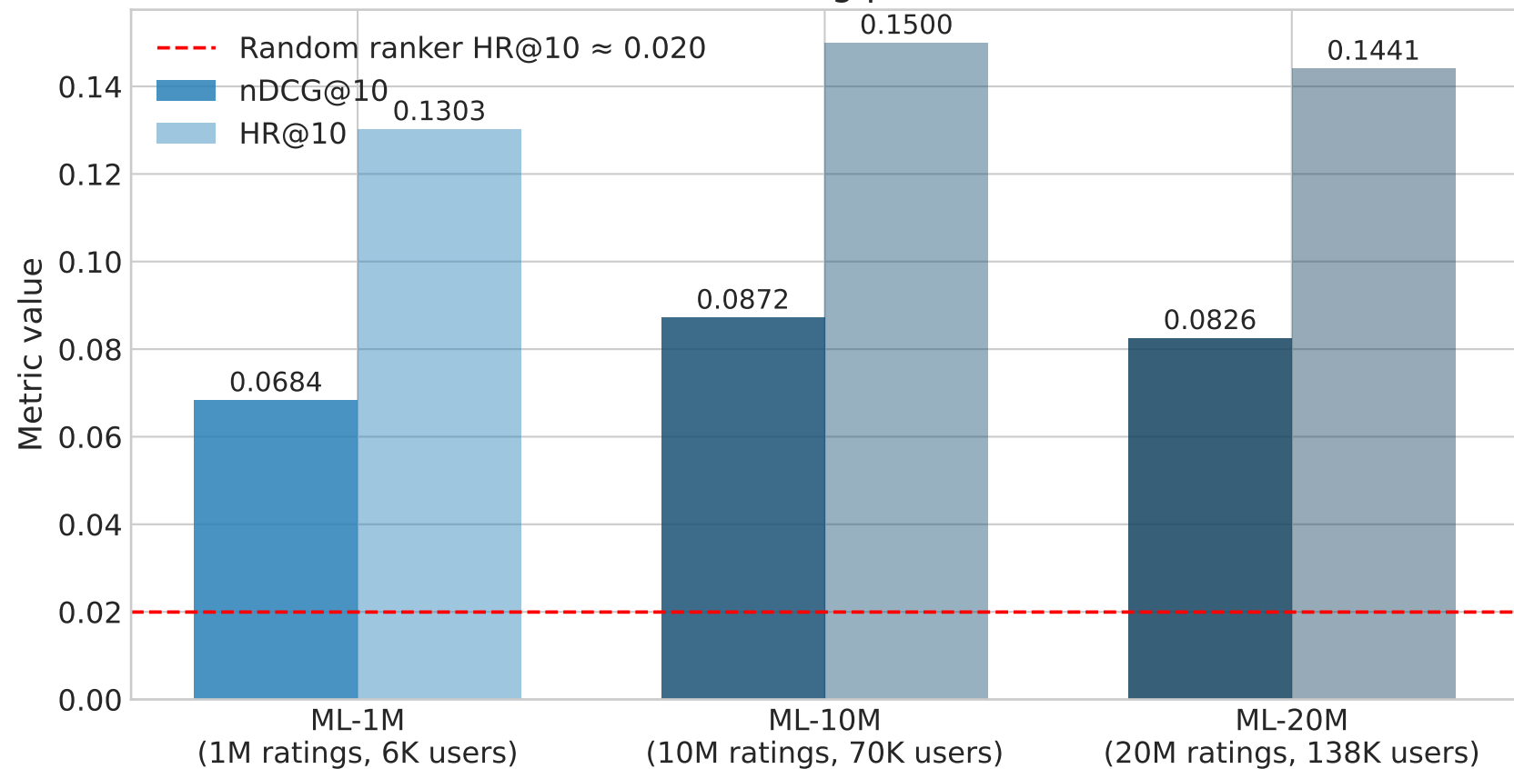
Baseline ranking performance
