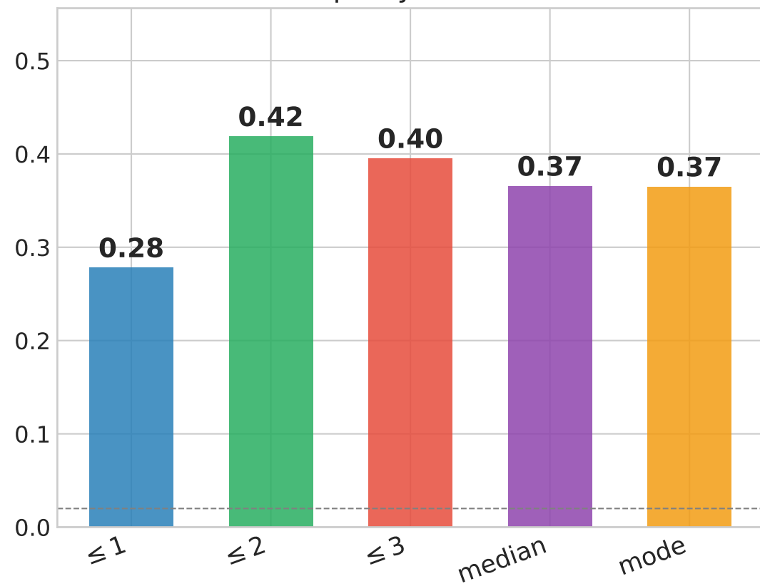
Spotify MSSD
