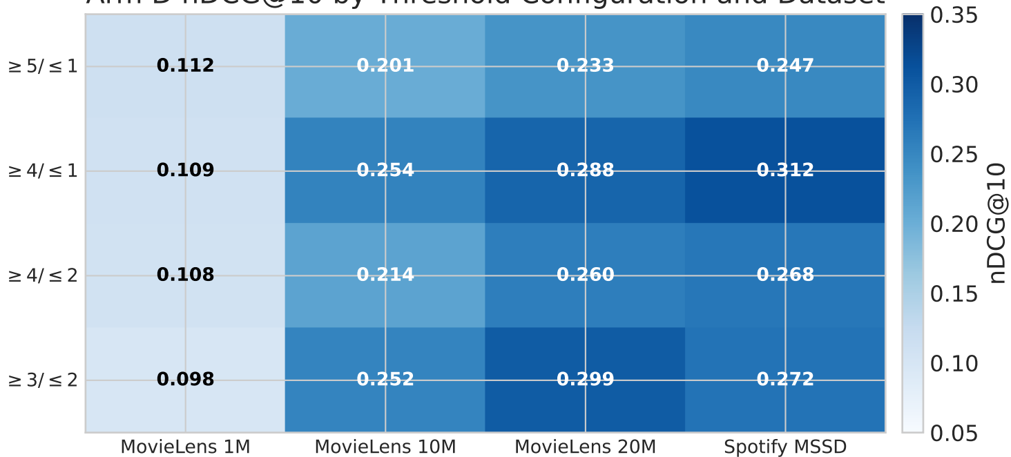
Arm D nDCG@10 by Threshold Configuration and Dataset
