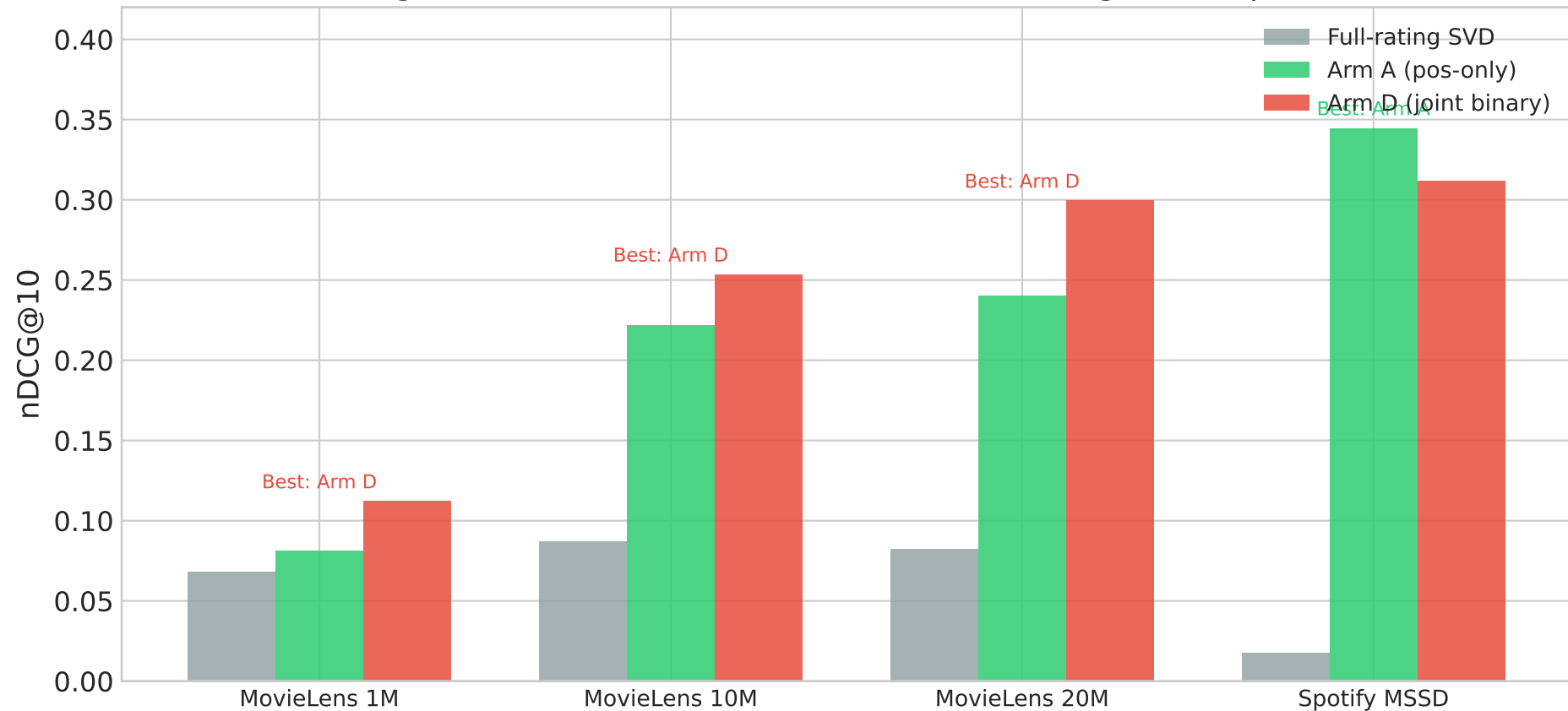
Full-rating SVD vs.\ Arm A vs.\ Arm D — Best Configuration per Dataset
