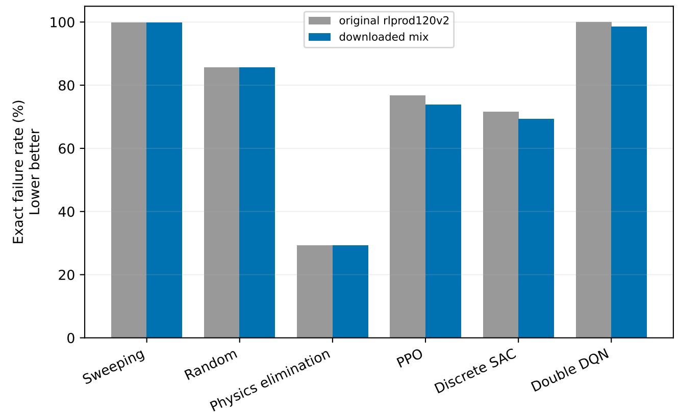
Downloaded `mix` FNO
