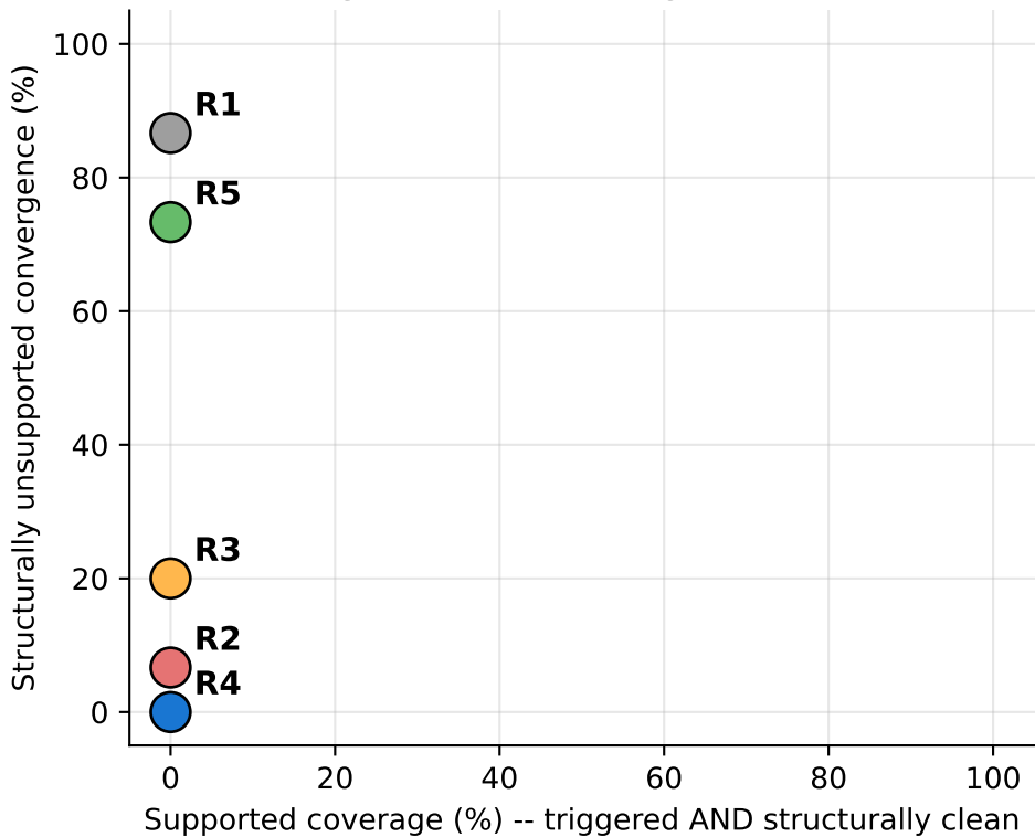
E6 F1 -- Coverage vs. overclaiming trade-off (N=15 cases)
