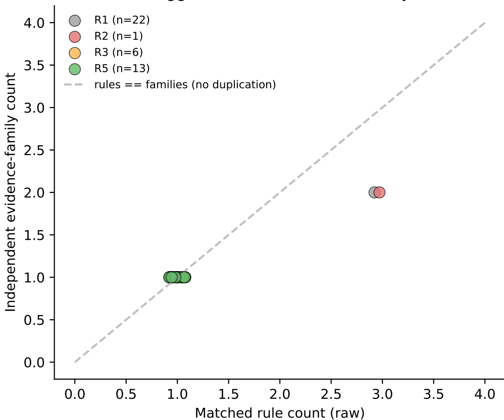
E6 F5 -- Raw rule count vs. independent family count (triggered domain-instances only)
