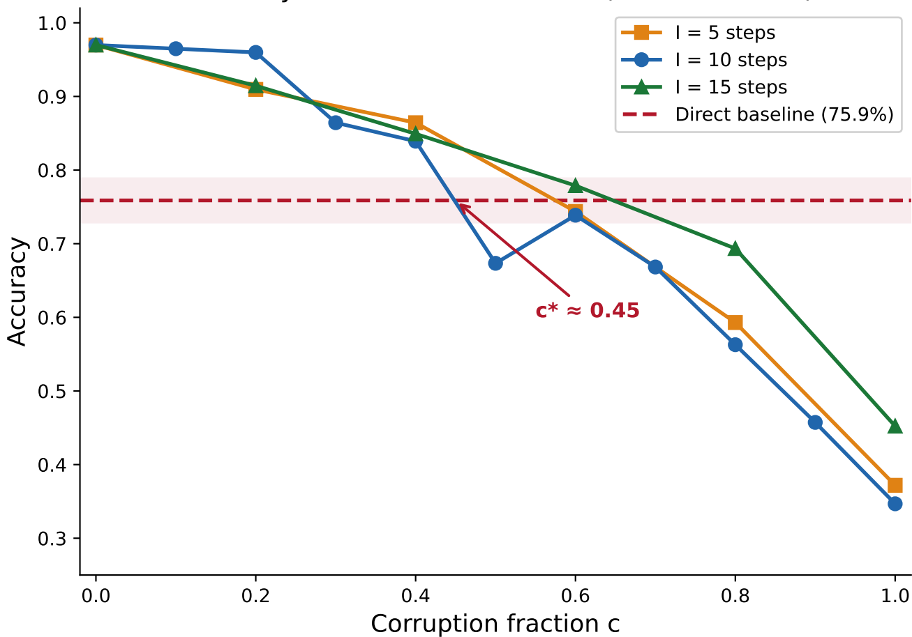
Accuracy Under Provided Traces (Claude Sonnet)
