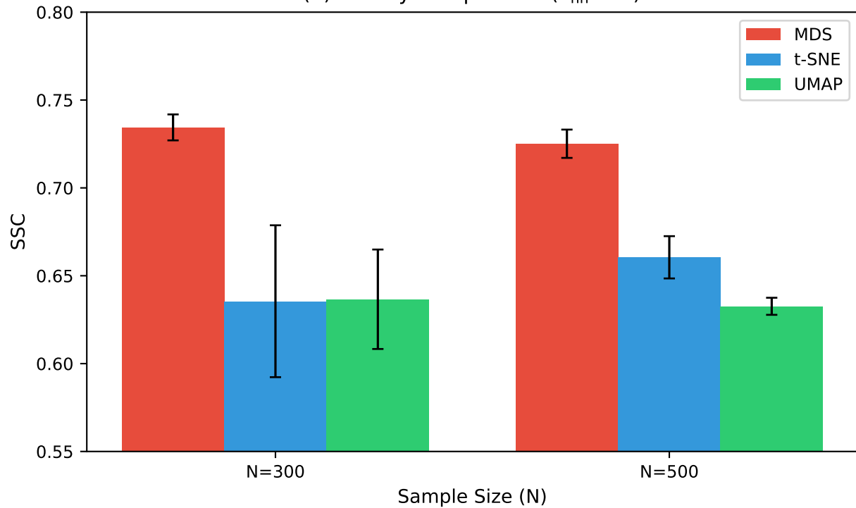
(b) SSC by Sample Size ( k_{nn}=10 )
