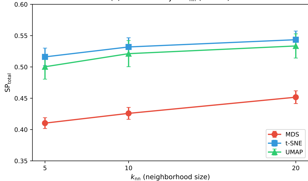
(a) SP Sensitivity to k_{nn} (N=500)
