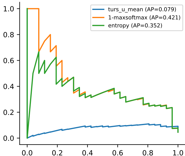
Error-detection PR — CWRU_BAL
