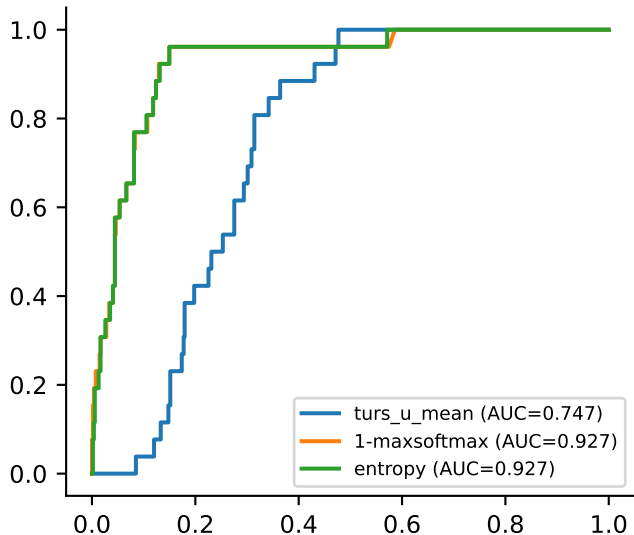
Error-detection ROC — CWRU_BAL
