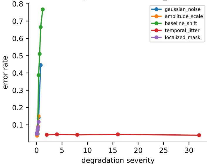
Severity vs error — CWRU_BAL
