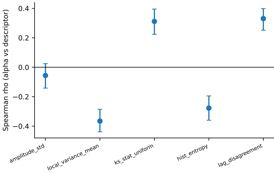
alpha vs independent input descriptors — CWRU_BAL
