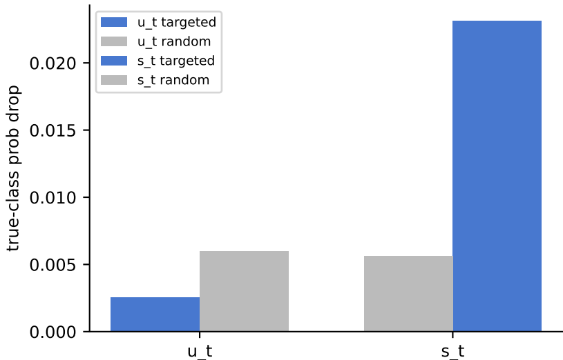
Faithfulness: targeted vs random — CWRU_BAL
