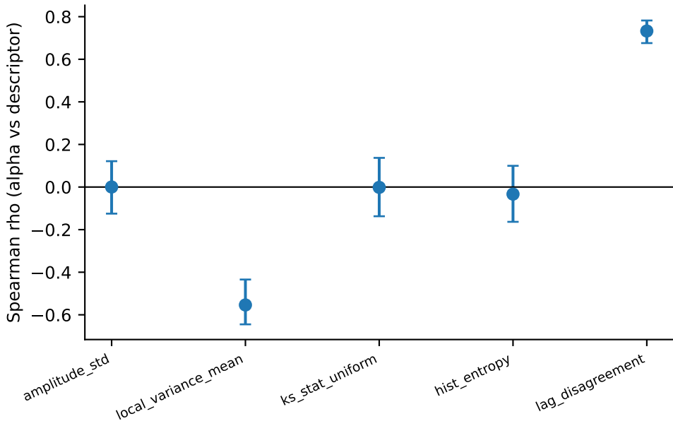
alpha vs independent input descriptors — CWRU_UNBAL
