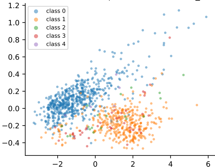
TURS-Lite latent z (pooled) — ECG5000_BAL
