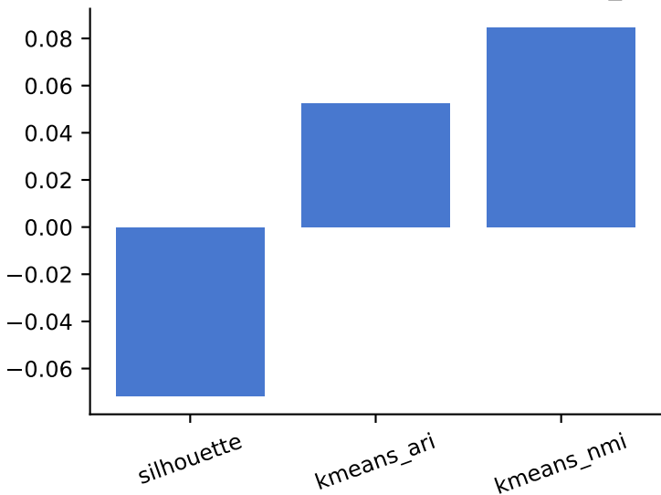
Latent class structure (test) — ECG5000_BAL
