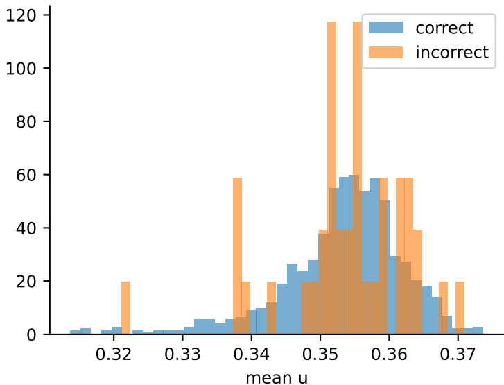
Uncertainty: correct vs incorrect — ECG5000_BAL
