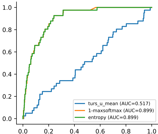
Error-detection ROC — ECG5000_BAL
