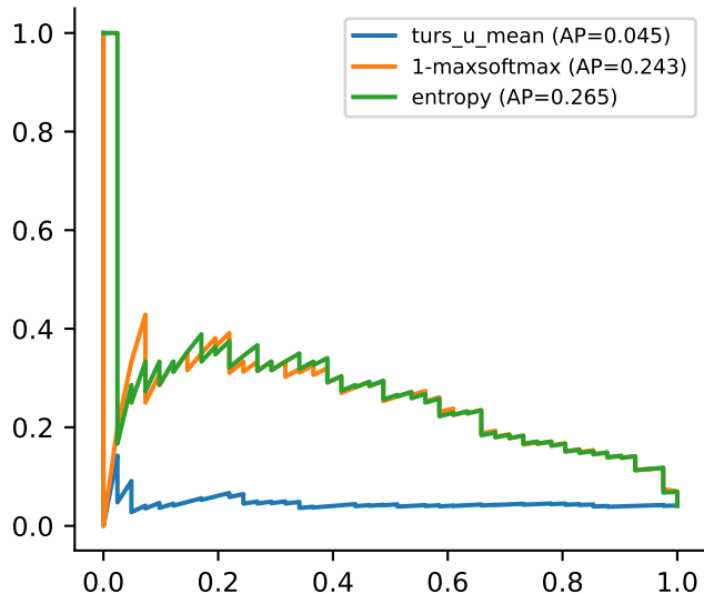
Error-detection PR — ECG5000_BAL
